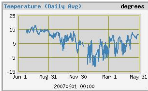
Fig. 6. Plot of the daily average temperature ( ^{\circ}\text{C} ) recorded at SPM (1.5-m telescope) for the period June 2006 to May 2007.
