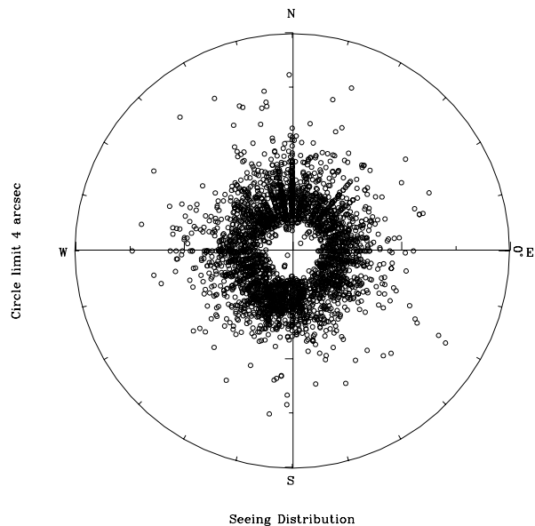
Fig. 17. Seeing as a function of wind direction, excluding measurements under high wind speeds (lower than around 30 \text{ km h}^{-1} ). From Echevarría et al. (1998).
