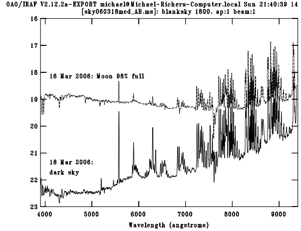
Fig. 12. Sky brightness on an AB magnitude scales as a function of wavelength. The data were obtained using the Boller & Chivens spectrograph. The spectral resolution is about 9Å.
